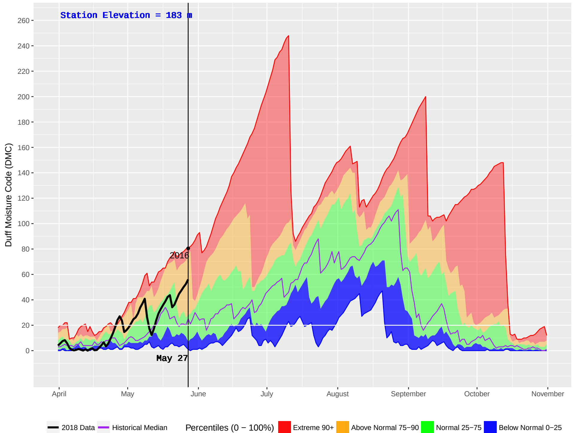
MESACHIE 2 (934) : Historical (2006–2016) and Current (2018) Noon Duff Moisture Code (DMC)
