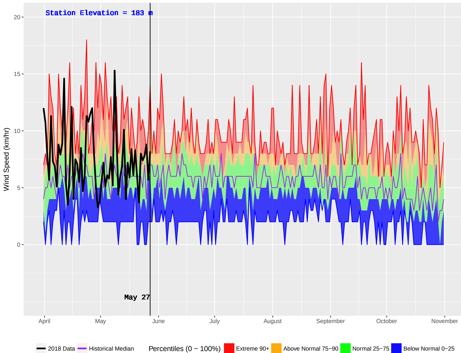
MESACHIE 2 (934) : Historical (2006–2016) and Current (2018) Noon Wind Speed
