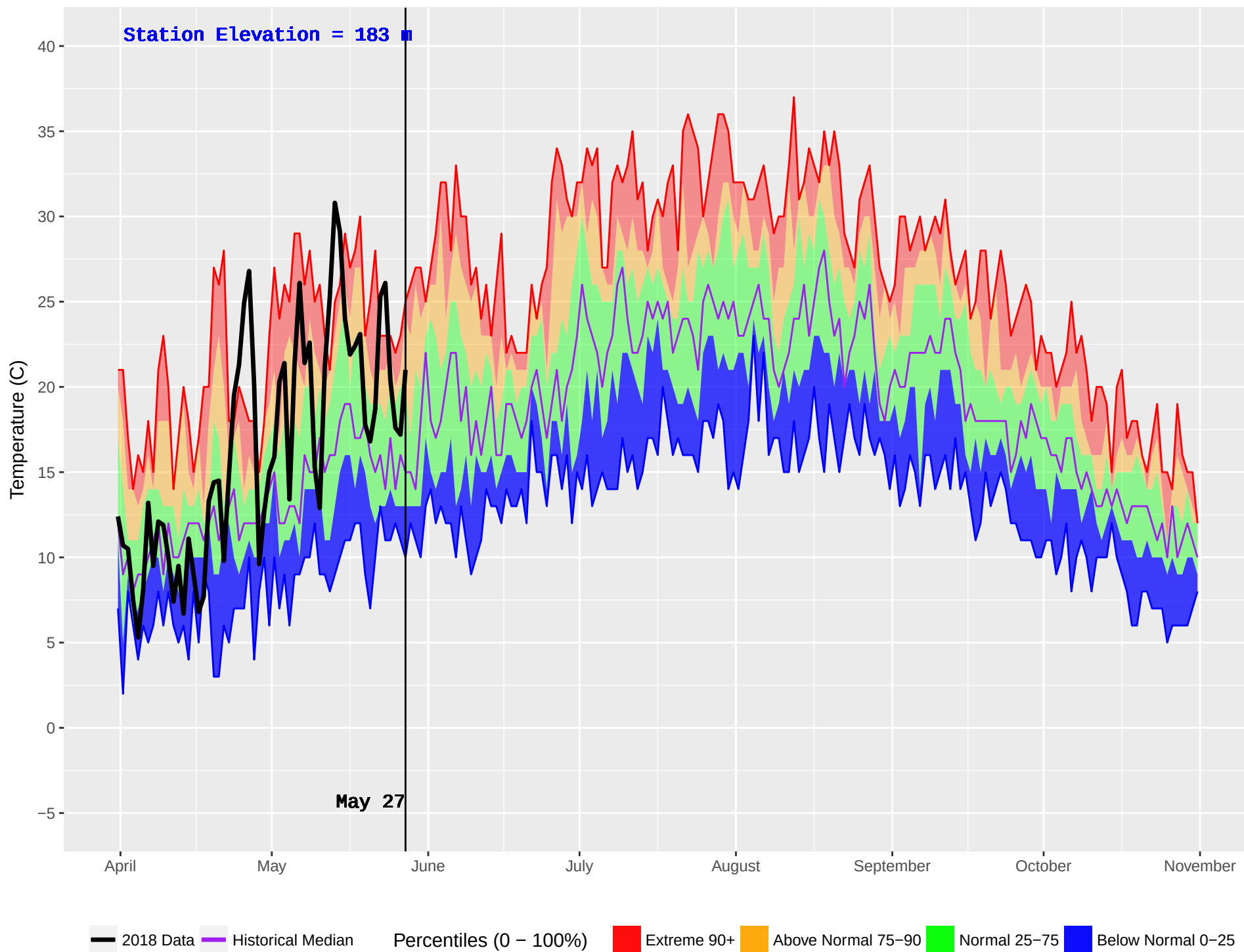
MESACHIE 2 (934) : Historical (2006–2016) and Current (2018) Noon Temperature
