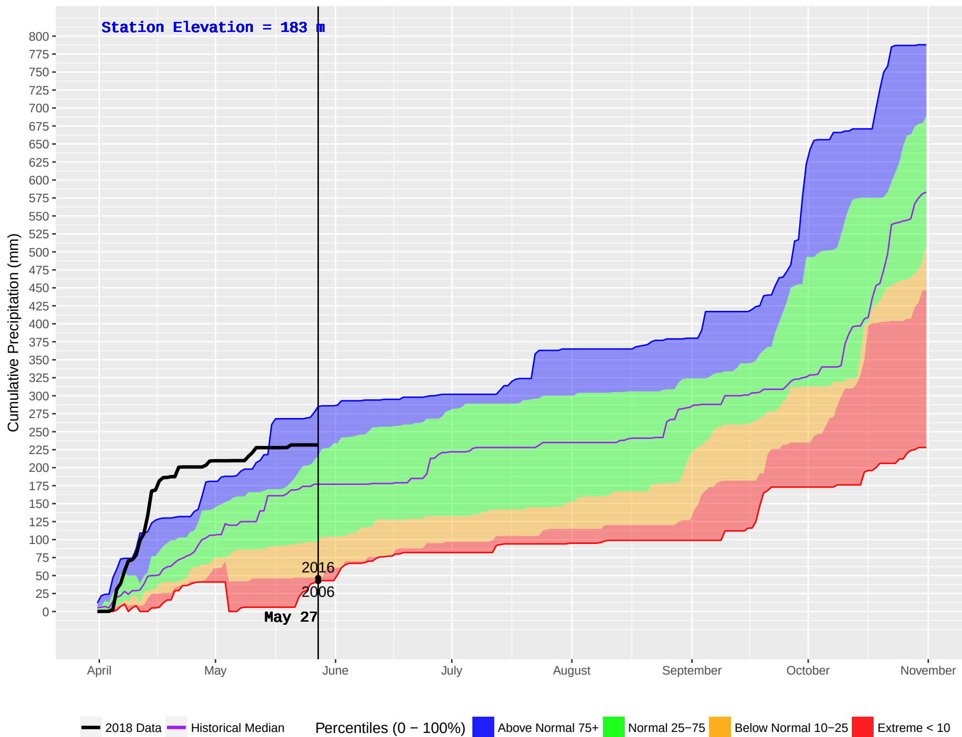
MESACHIE 2 (934) : Historical (2006–2016) and Current (2018) Noon Cumulative Precipitation
