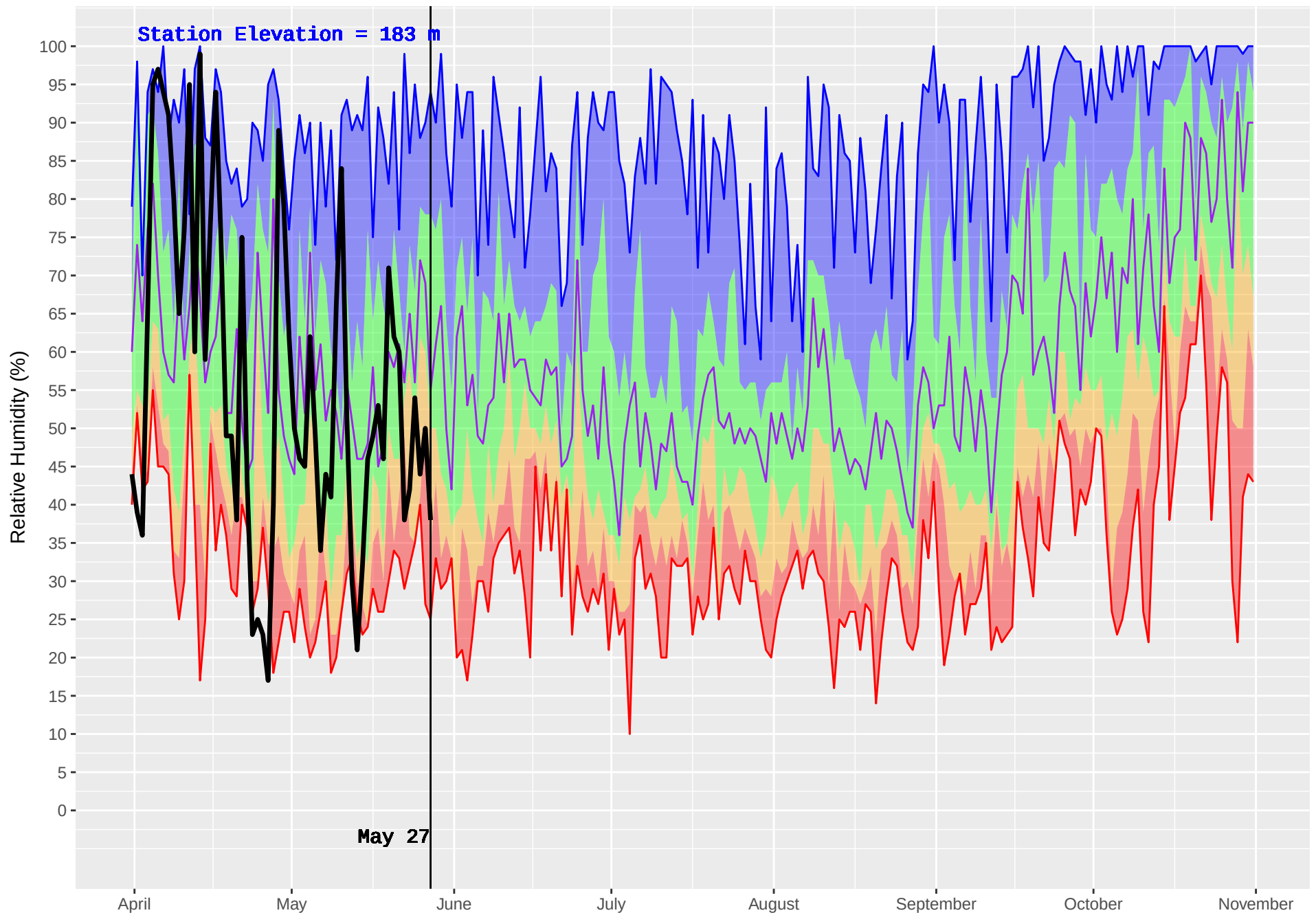
MESACHIE 2 (934) : Historical (2006–2016) and Current (2018) Noon Relative Humidity
