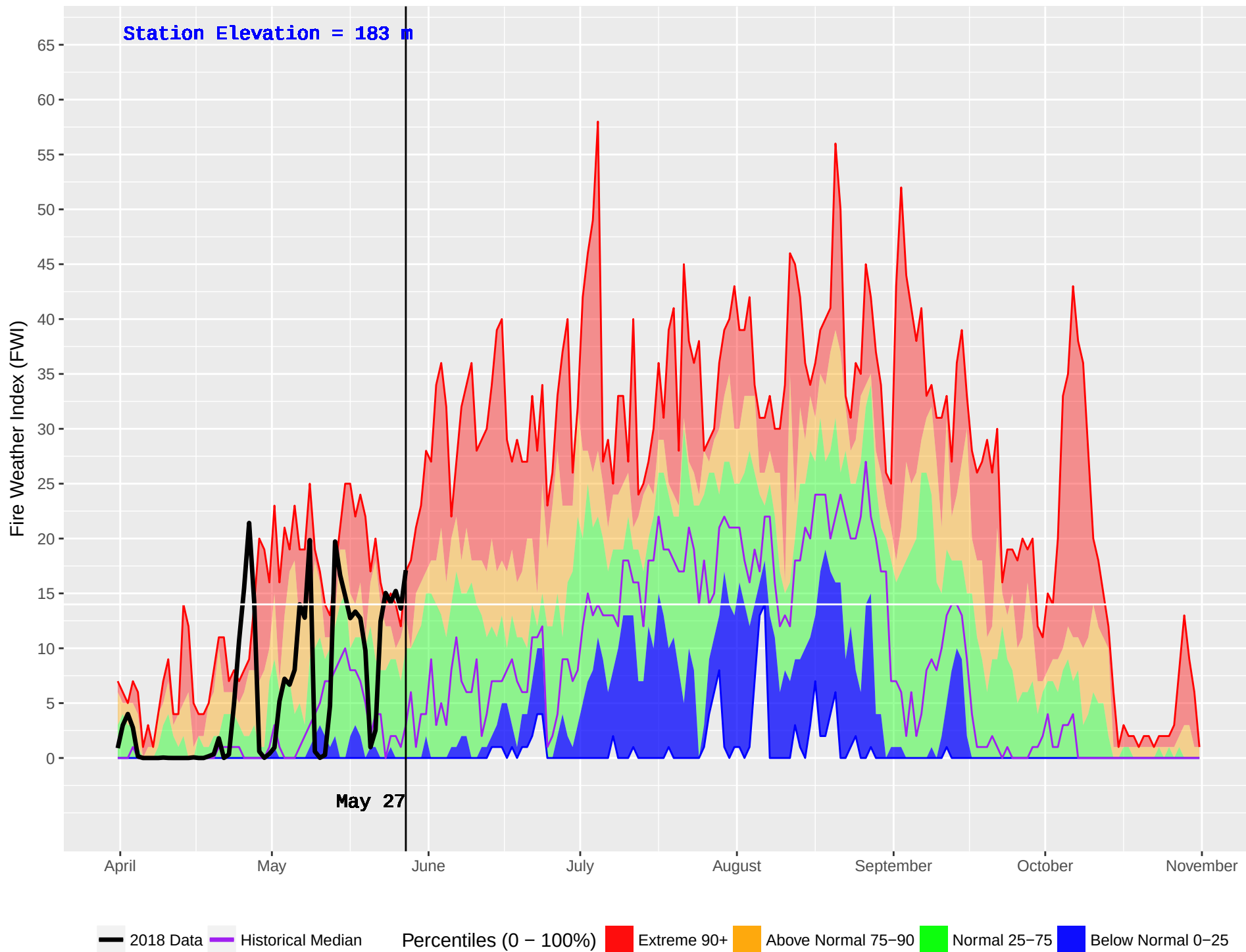
MESACHIE 2 (934) : Historical (2006–2016) and Current (2018) Noon Fire Weather Index (FWI)
