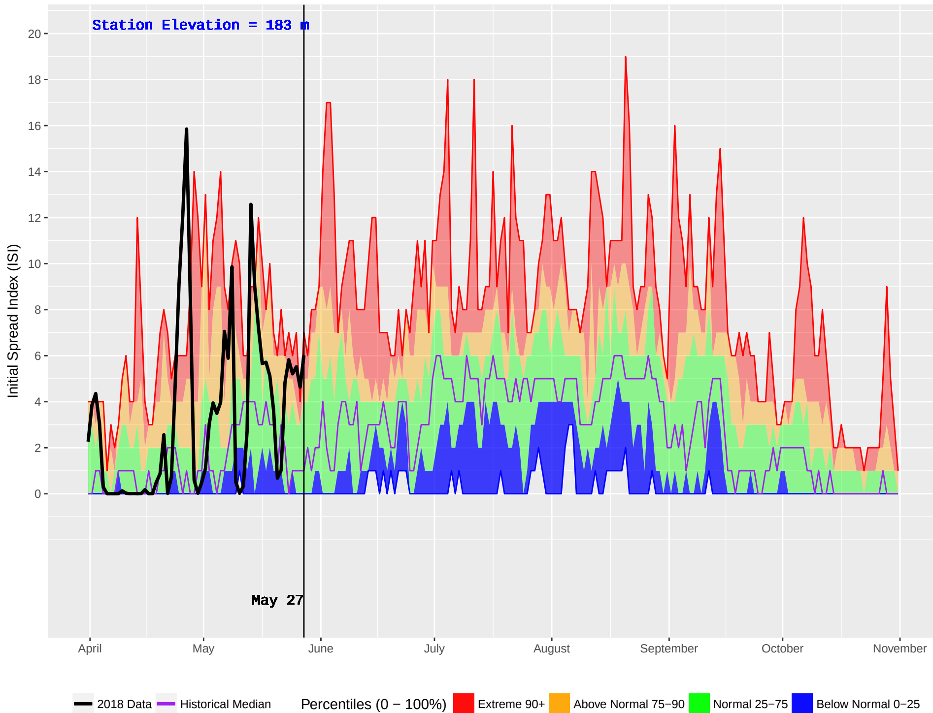
MESACHIE 2 (934) : Historical (2006–2016) and Current (2018) Noon Initial Spread Index (ISI)
