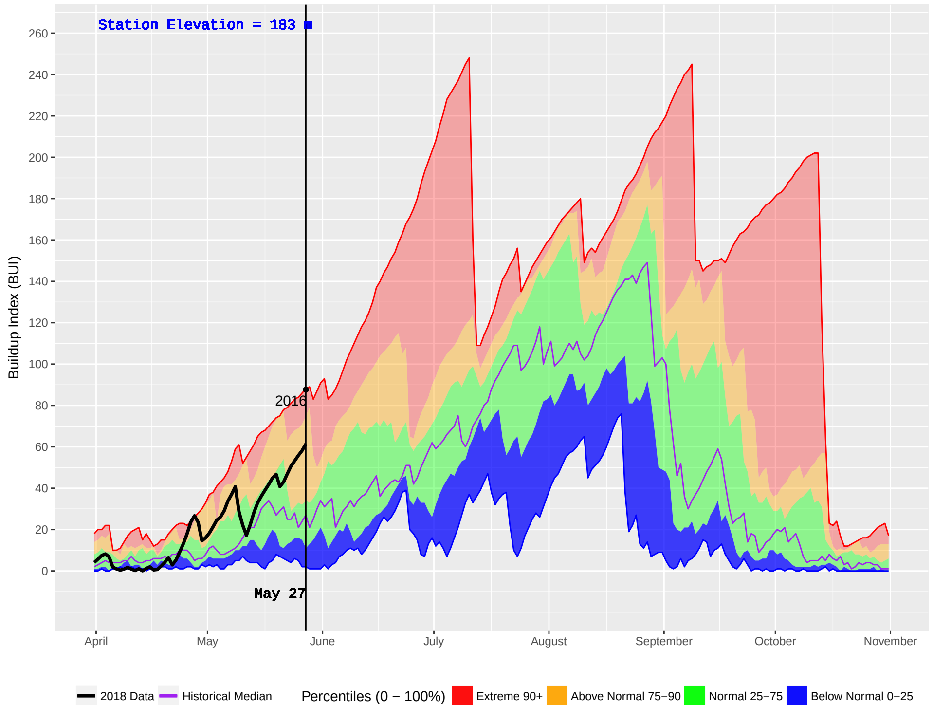
MESACHIE 2 (934) : Historical (2006–2016) and Current (2018) Noon Buildup Index (BUI)
