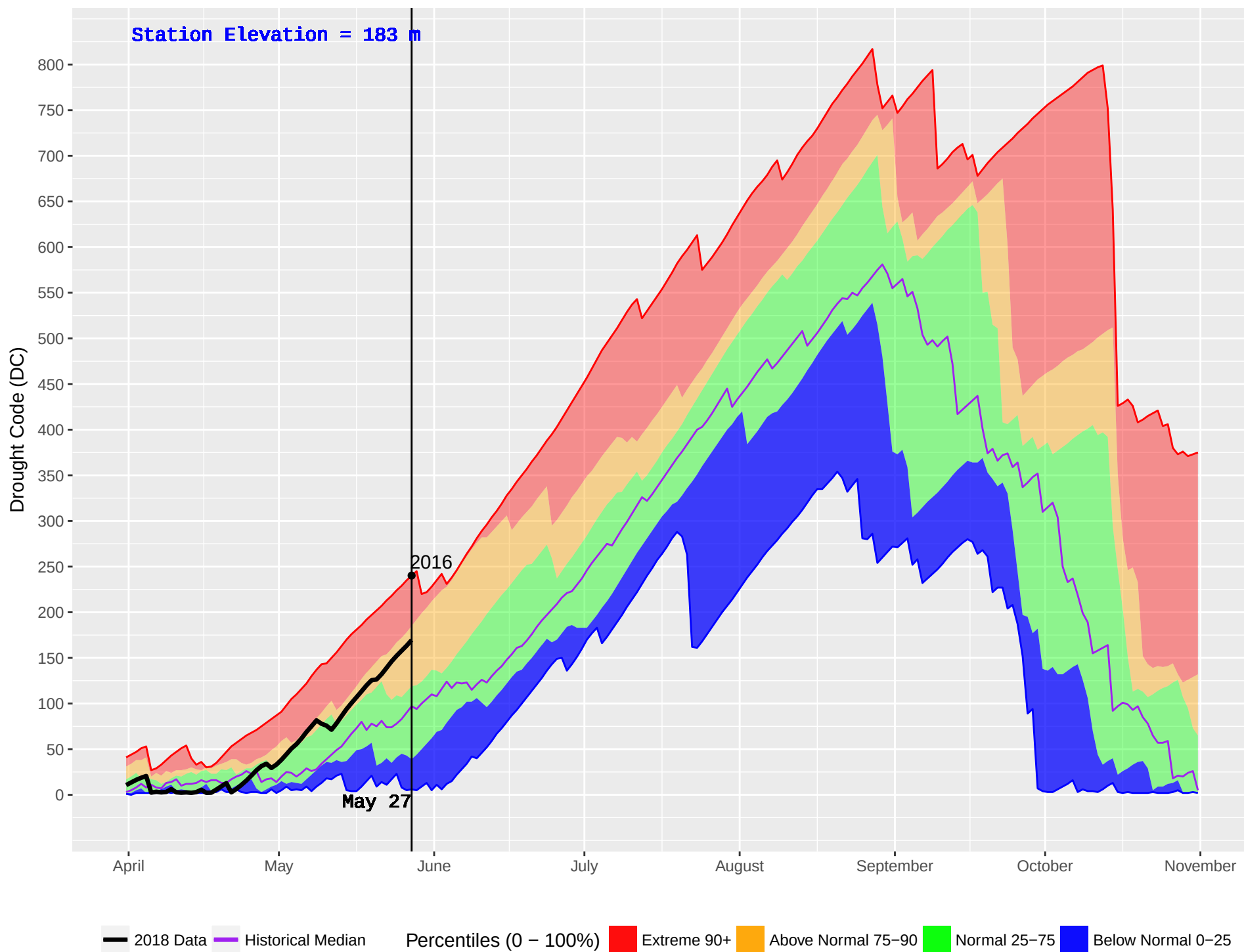
MESACHIE 2 (934) : Historical (2006–2016) and Current (2018) Noon Drought Code (DC)
